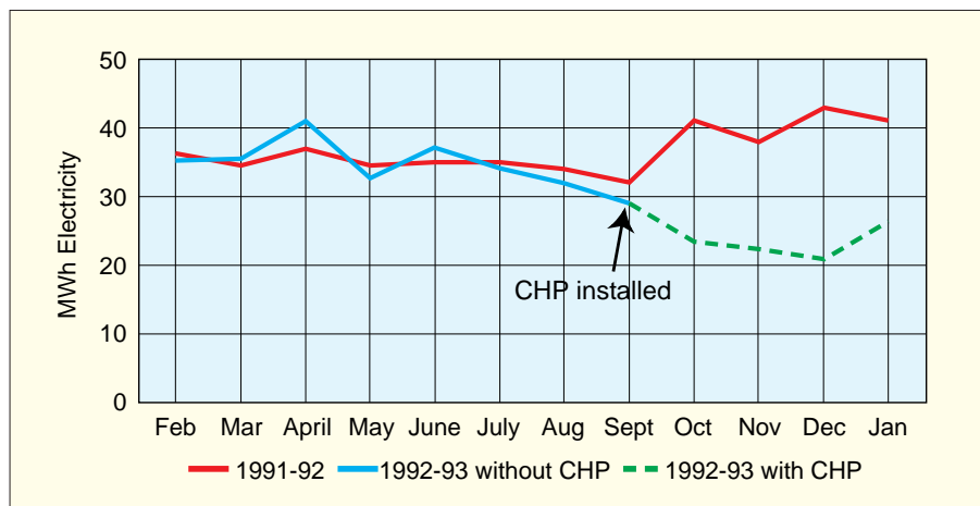
Figure 6 Power purchased from REC for the Posthouse Grimsby
