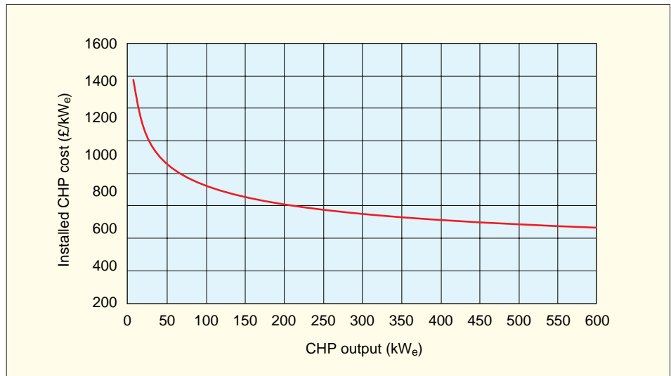
Figure 4 Typical installed costs for small-scale packaged CHP units
